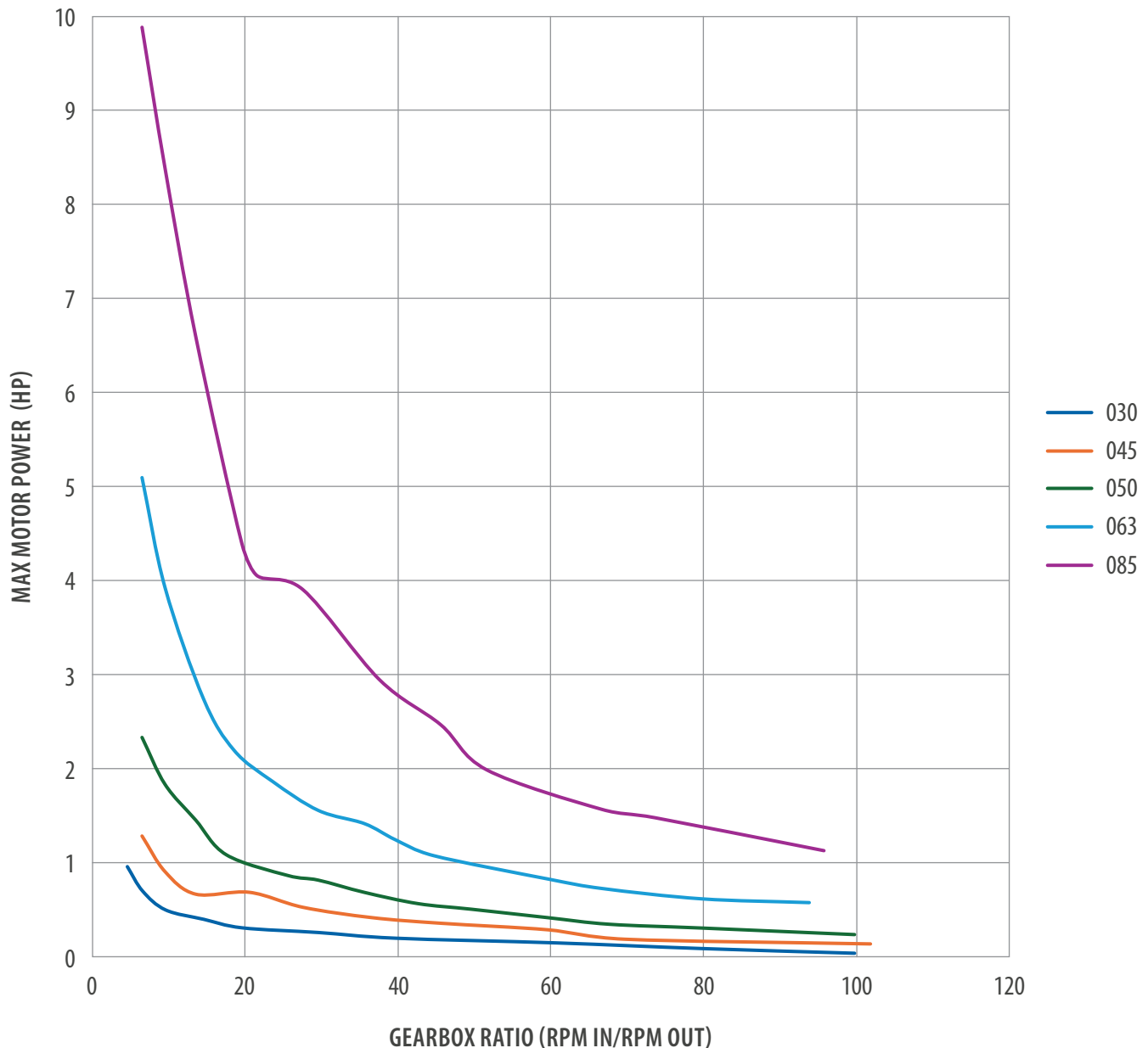
Max Motor Power vs Ratio (ALRN)
