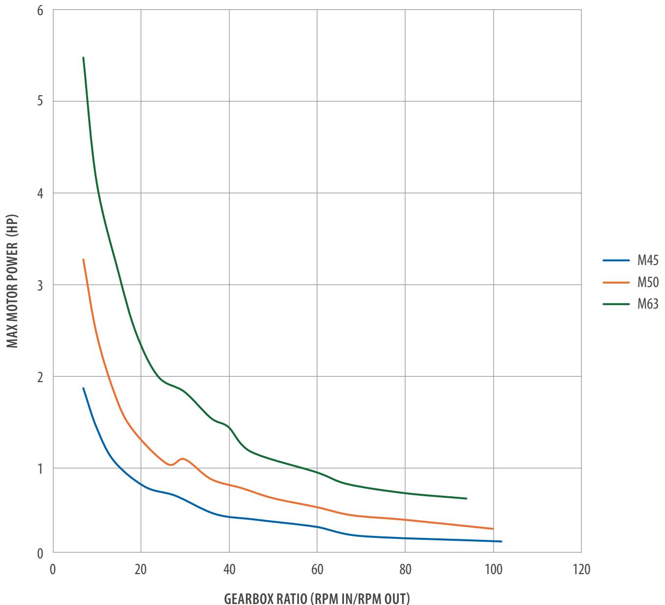
Max Motor Power vs Ratio (ALSQ)
