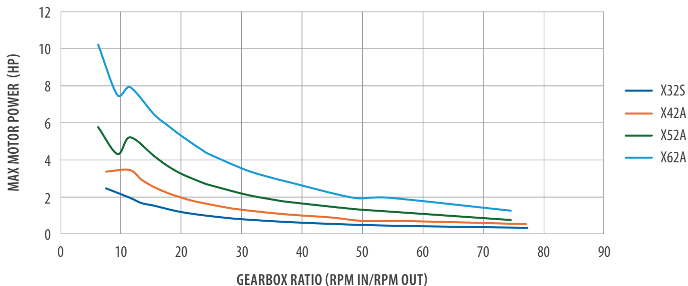
Max Motor Power vs Ratio 2 Stage (HXB)
