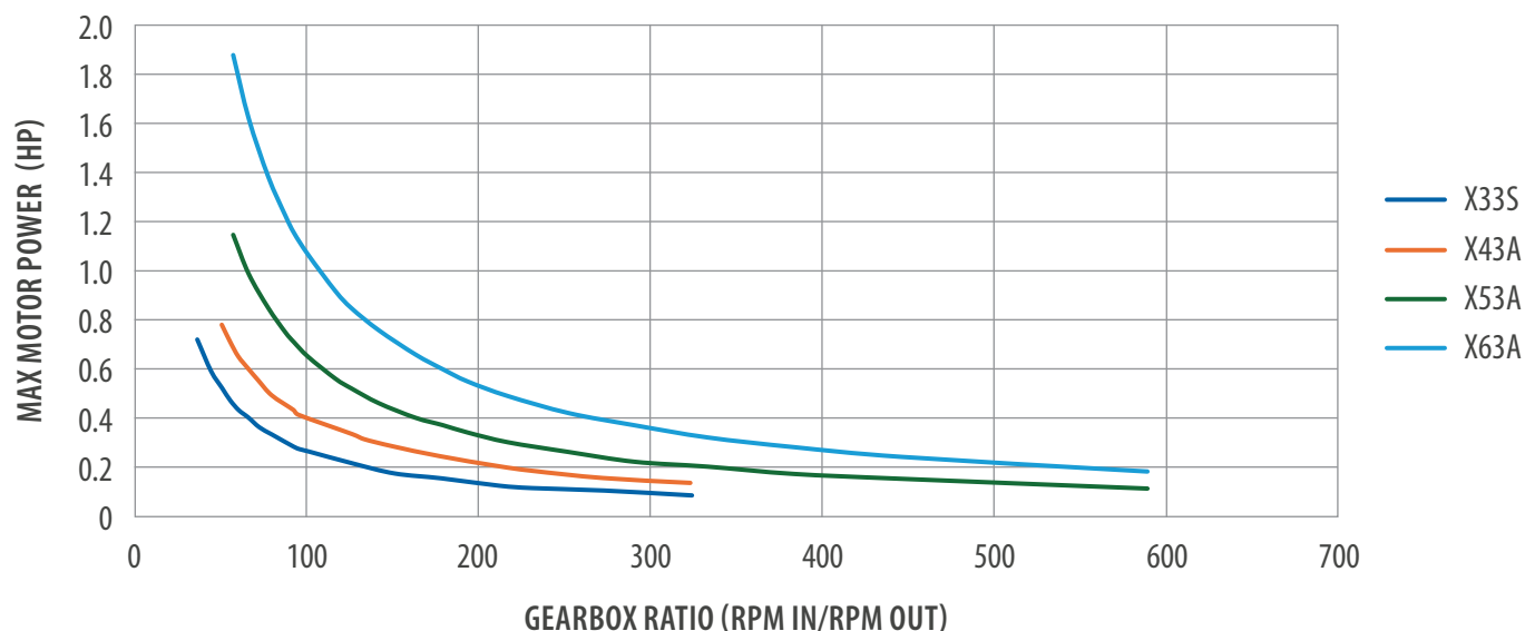
Max Motor Power vs Ratio 3 Stage (HXB)
