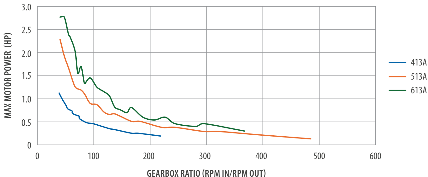
Max Motor Power vs Ratio 3 Stage (HXI)
