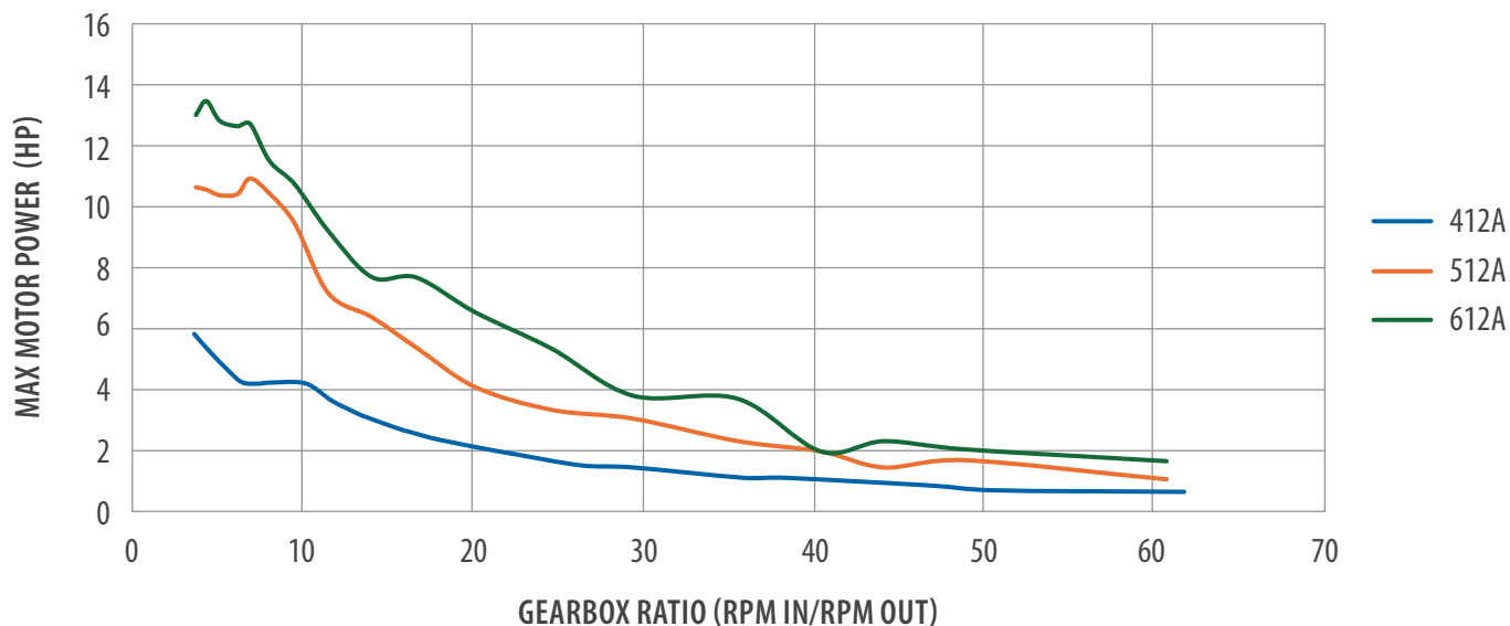
Max Motor Power vs Ratio 2 Stage (HXI)
